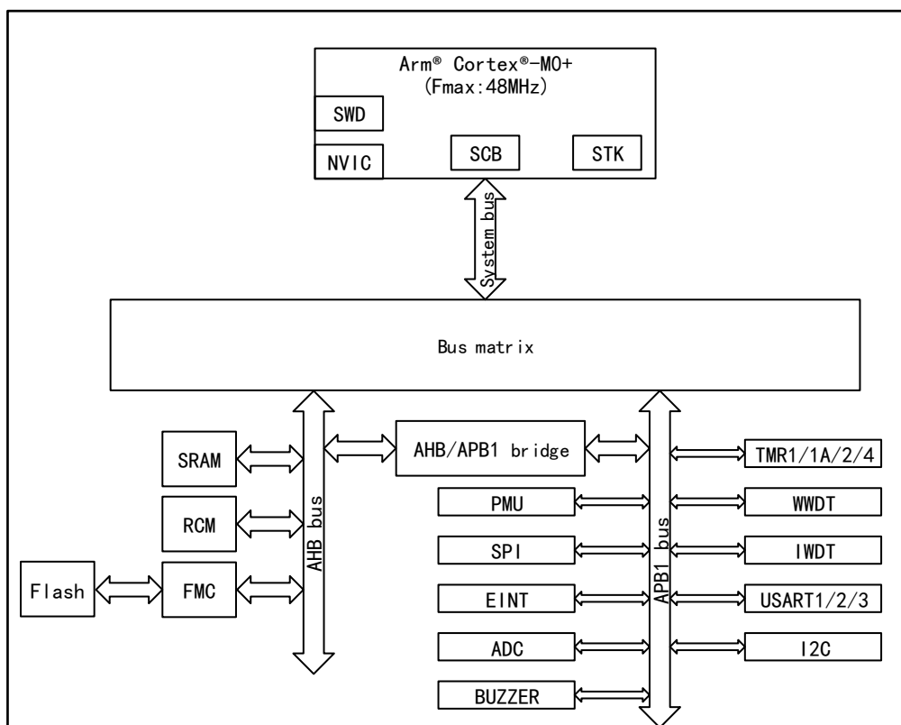
Figure 2 System block diagram of APM32A003F6Ux series
