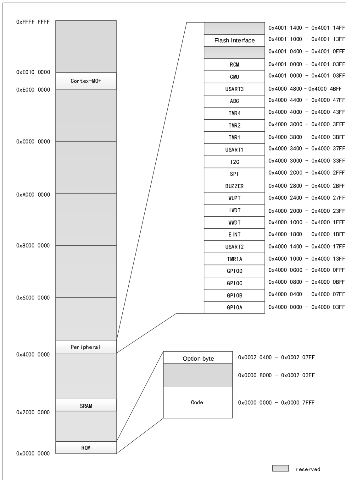
Figure 3 Address map of APM32A003F6Ux series
