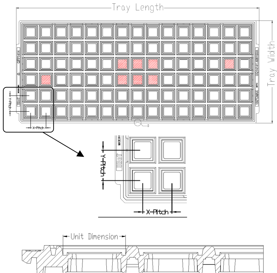
Figure 15 Tray Dimensions
