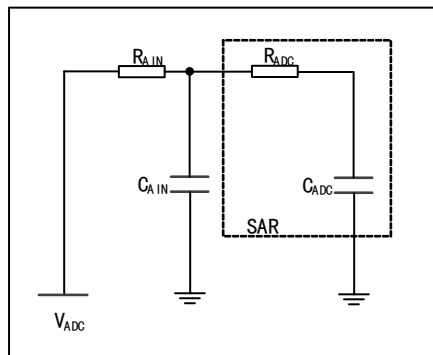
Figure 11 Typical application of ADC
