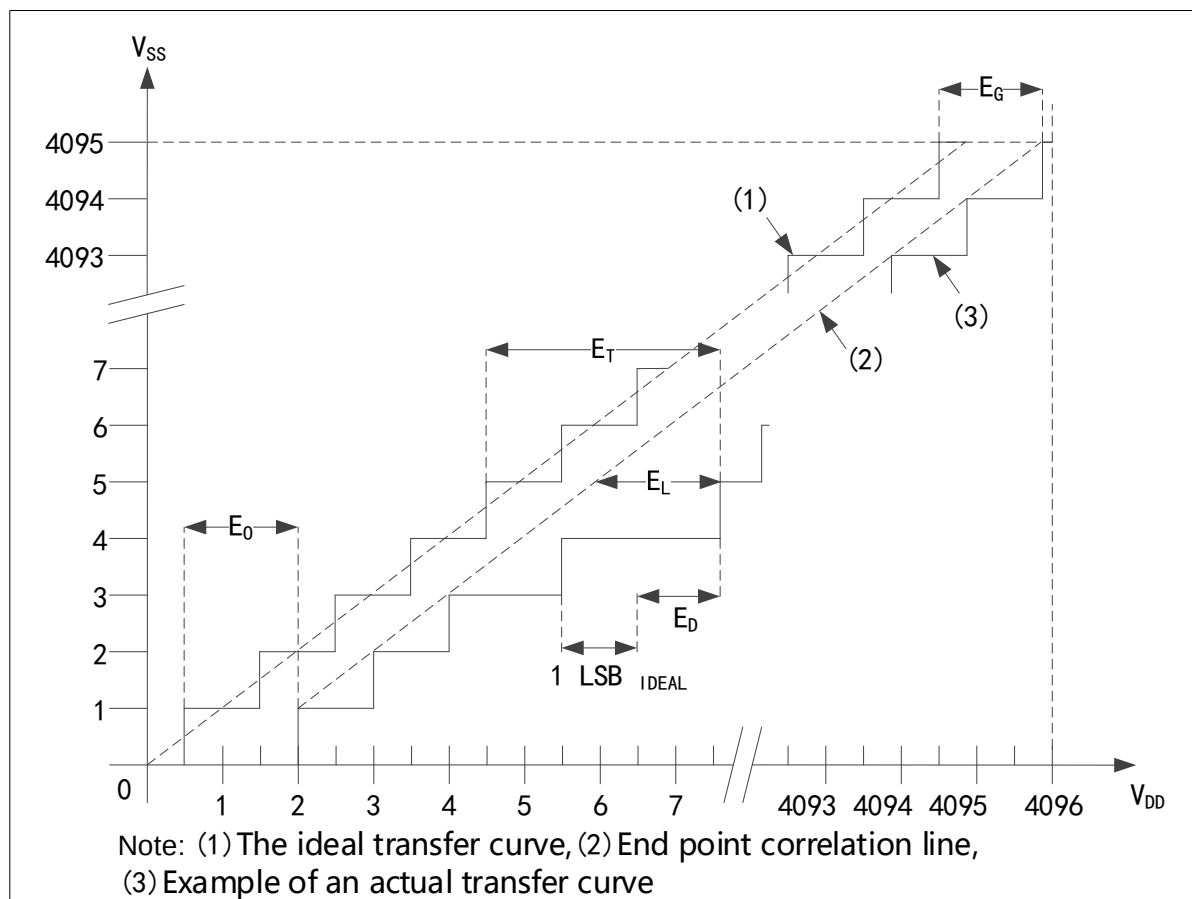
Figure 12 ADC Accuracy Characteristics
